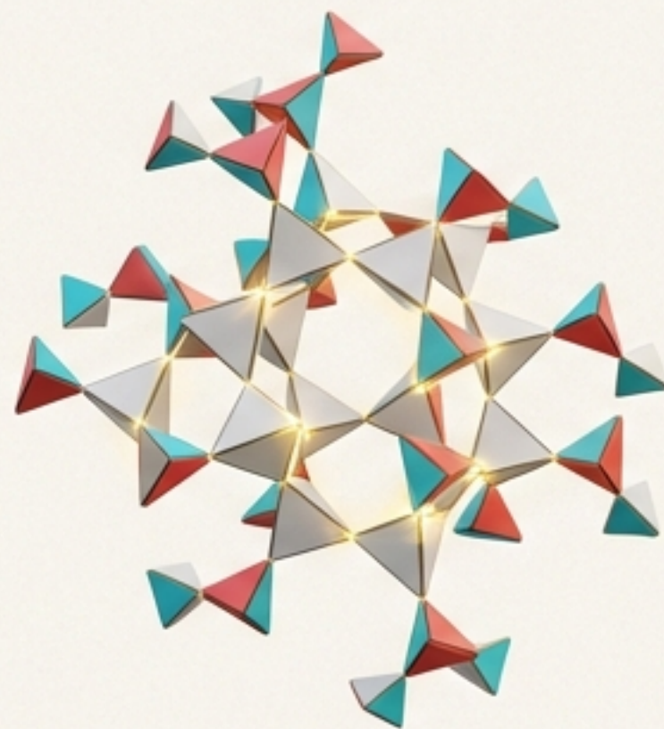
ENERGY: \text{C}_6\text{H}_{12}\text{O}_6
